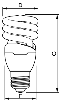
QSPIR-F Erp 15W/827 E27 220-240V 50/60Hz
