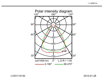
IFPC_4MX900 G3 581 1xLED40S/840 PSU MB-Polar Indoor (combined)
