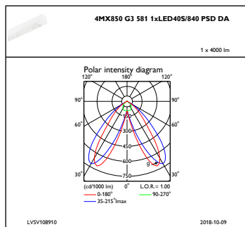
IFPC1_4MX850G35811xLED40S840PSDDA
