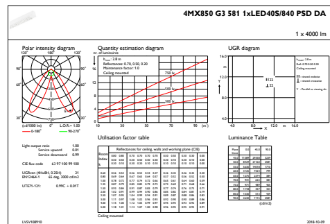
IFGU1_4MX850G35811xLED40S840PSDDA
