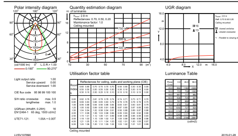
IFGU_4MX400 G3 491 1xLED40S/840 PSD NB-General uniform lighting
