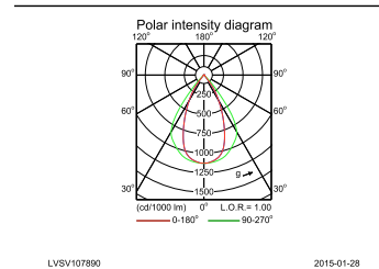
IFPC_4MX400 G3 491 1xLED40S/840 PSD NB-Polar Indoor (combined)
