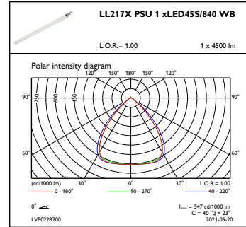
OFPC1_LL217XPSU1xLED45S840WB
