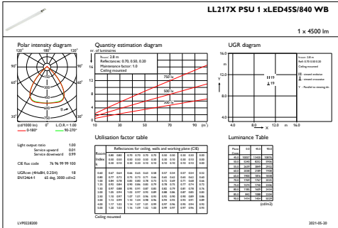
IFGU1_LL217XPSU1xLED45S840WB
