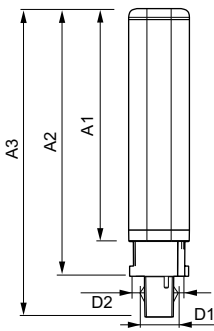
PLED PLC 230V 5W 450lm 3000K G24D-1 ND
