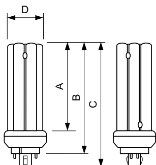
PL-T 18W/827/4P M
