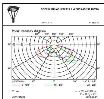
OFPC1_BDP794MK-WHFGT251xLED53-4S740DW10
