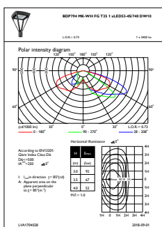
OFPL1_BDP794MK-WHFGT251xLED53-4S740DW10
