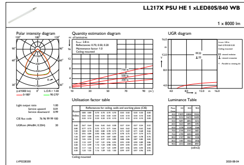
IFGU1_LL217XPSUHE1xLED80S840WB
