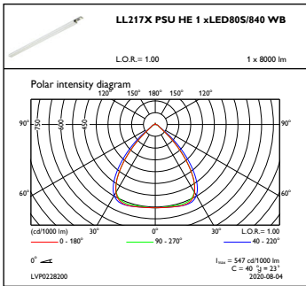
OFPC1_LL217XPSUHE1xLED80S840WB
