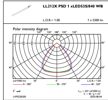
OFPC1_LL212XPSD1xLED53S840WB
