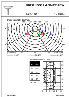
OFPL1_BDP101PCC1xLED40830DW
