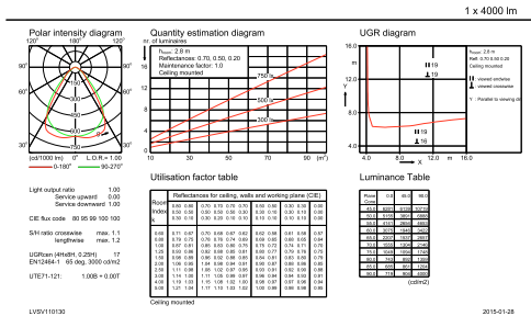
4MX900 G3 581 1xLED40S/840 PSU MB
