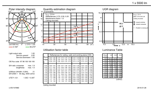
IFGU_4MX400 G3 491 1xLED55S/840 PSD WB- General uniform lighting
