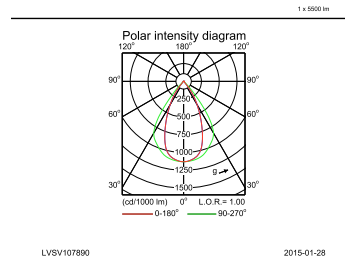
IFPC_4MX400 G3 491 1xLED55S/840 PSD NB-Polar Indoor (combined)
