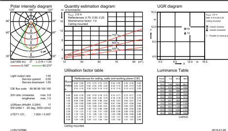
IFGU_4MX400 G3 491 1xLED55S/830 PSD NB-General uniform lighting
