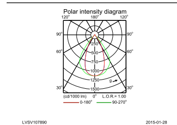
IFPC_4MX400 G3 491 1xLED55S/830 PSD NB-Polar Indoor (combined)
