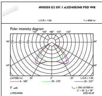
OFPC1_4MX850G35811xLED40S840PSDWB
