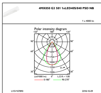
IFPC1_4MX850G35811xLED40S840PSDNB
