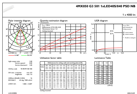
IFGU1_4MX850G35811xLED40S840PSDNB
