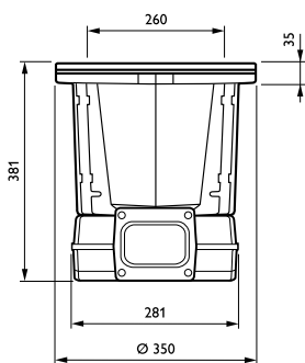
BBP623 34xLED-HB/NW I A GC GR RMR
