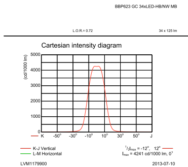
OFCC_BBP623 GC 34xLED-HB/NW MB-Cartesian Outdoor (combined)
